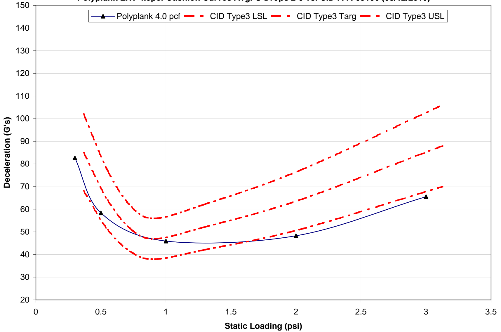
Polyplank EXT 4.0pcf Cushion Curves Avg. G Drops 2-5 vs. CID-A-A-59136 (08/12/2010)
